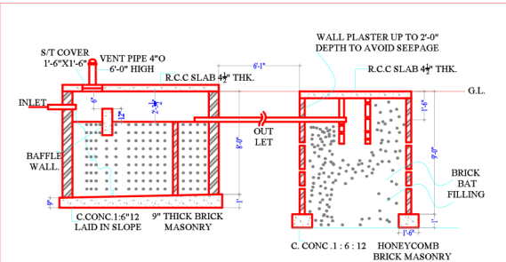
SECTION AT X-X'
