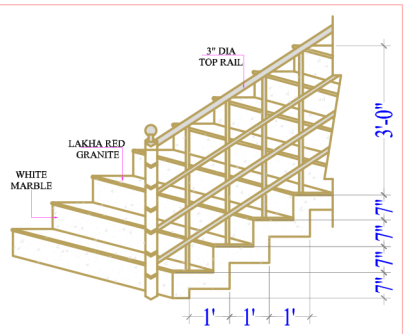
STAIRCASE DETAIL
